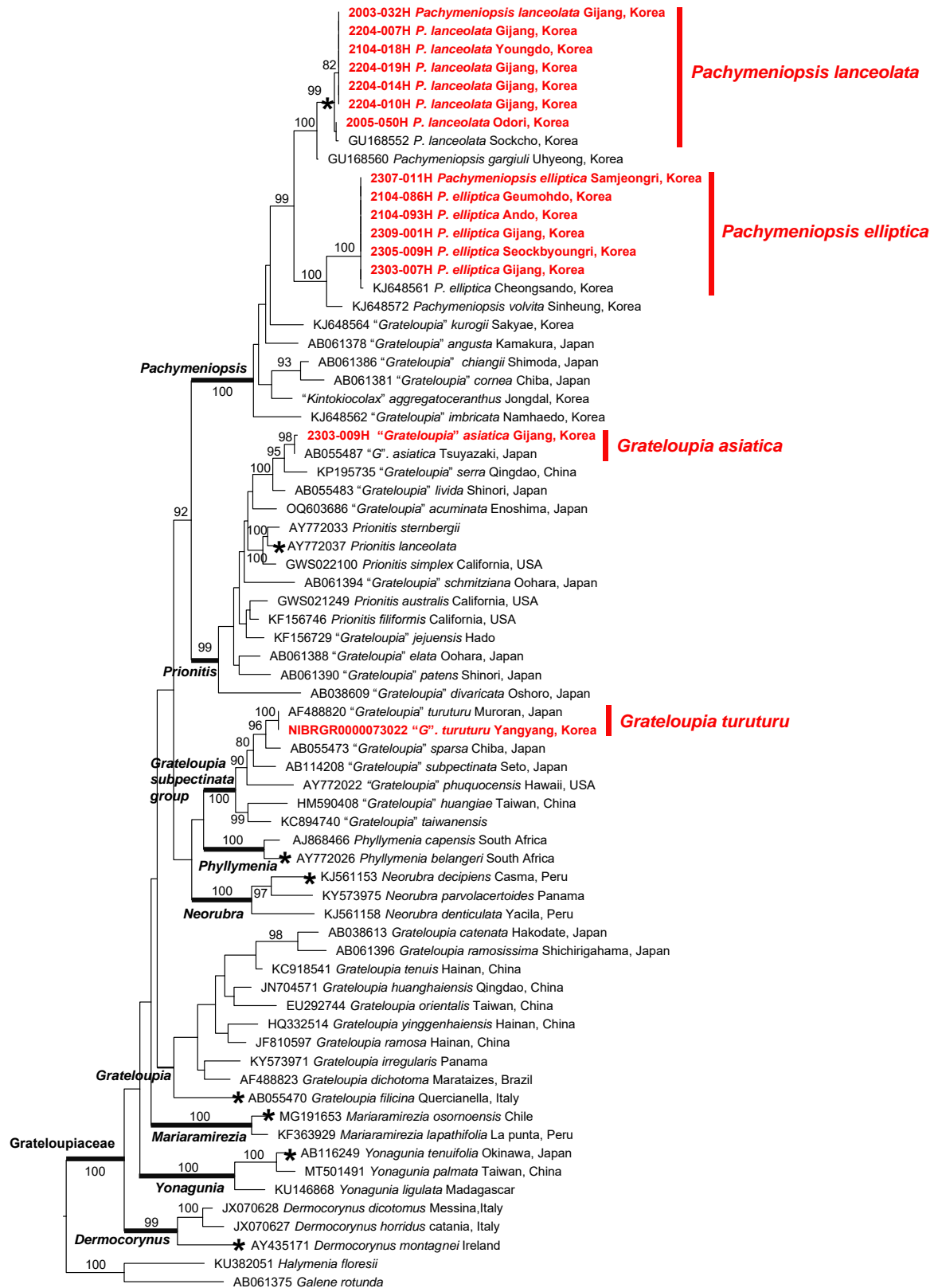
Supplementary Fig. S1. Maximum likelihood tree of Grateloupiaceae based on rbcL sequences. Red color indicates the host species of Reinboldiella koreana . The taxa in bold indicate newly analyzed in this study. An Asterisk (*) indicates the type species for each genus.
