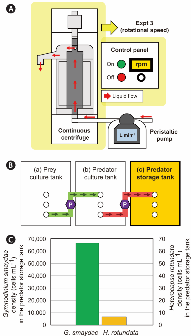
Supplementary Fig. S2. Schematic diagram showing the centrifuge used in the continuous centrifugation system (A), the water tank used in the semi-continuous cultivation system (B), and the densities of Gymnodinium smaydae and Heterocapsa rotundata cultivated and harvested for experiment 3 to determine the effects of the rotational speed of the continuous centrifuge on harvesting G. smaydae (C). P in B, the peristaltic pump transporting HR or GS culture to the predator culture or predator storage tank.
