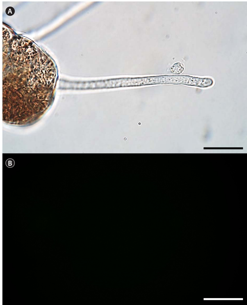
Supplementary Fig. S1. Inhibition of reactive oxygen species production during the fertilization of Bostrychia moritziana after treatment with 1 \mu\text{M} staurosporine. (A) Light microscopy image of staurosporine-treated spermatium attached to the trichogyne. (B) Fluorescence microscopy image of staurosporine-treated spermatium attached to the trichogyne after DCFH-DA staining. Scale bars represent: A & B, 20 \mu\text{m} .
