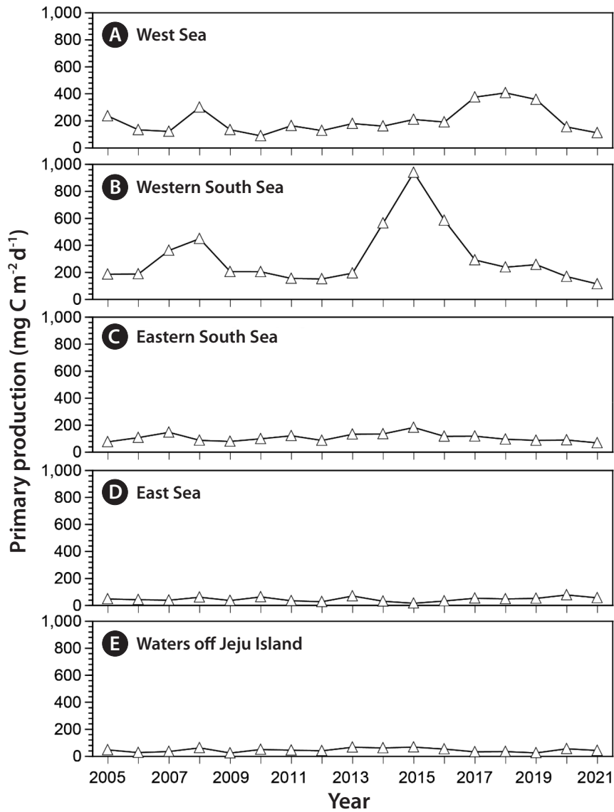
Supplementary Fig. S1. Long-term trend of primary production in each region.
