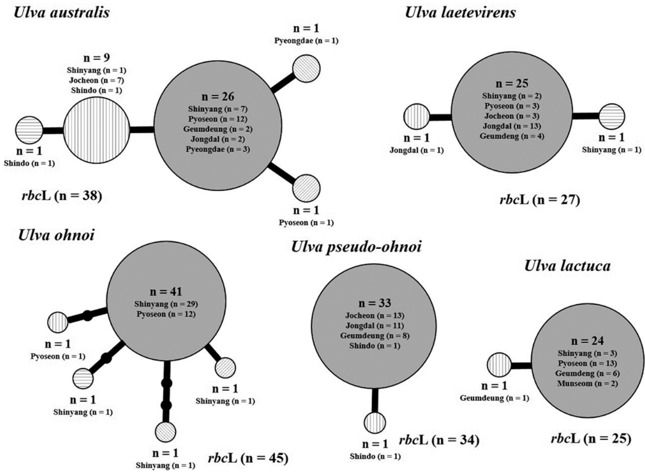
Supplementary Fig. S1. Statistical parsimony haplotype networks of rbcL marker generated in TCS within each Ulva blooming species from Jeju Island, Korea. Each haplotype is represented by a circle, and the size of each circle is proportional to the number of individuals with that haplotype.
