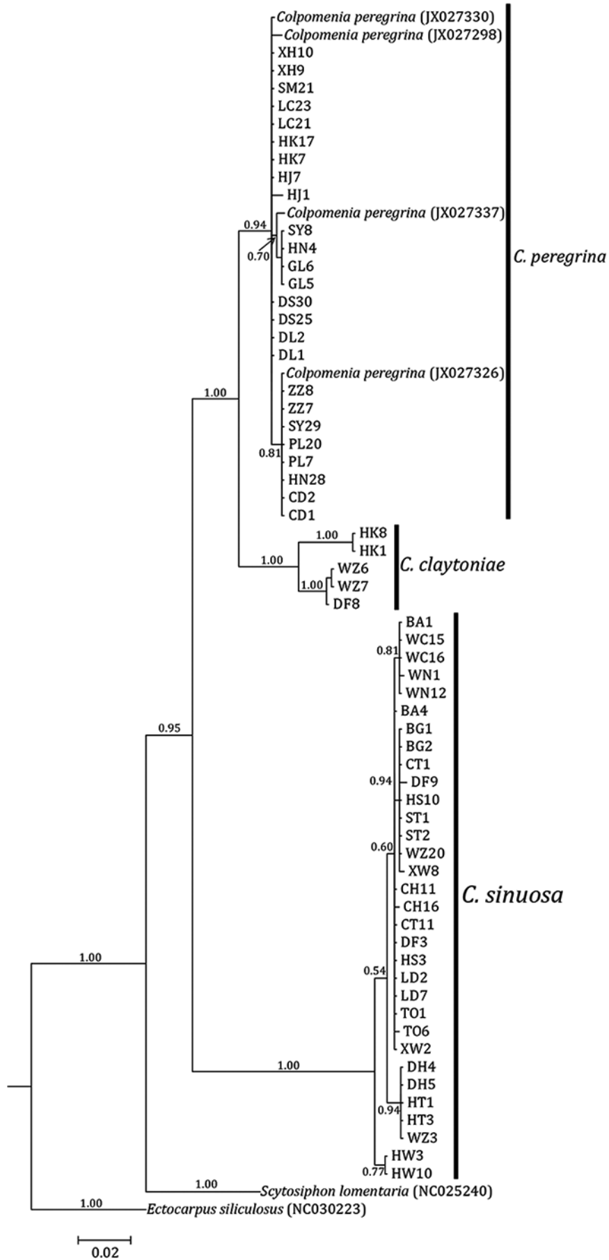
Supplementary Fig. S4. The Bayesian inference (BI) tree derived from atp6 sequences of Colpomenia . Numbers above or near branches are BI posterior probabilities. Values <0.50 were not shown.
